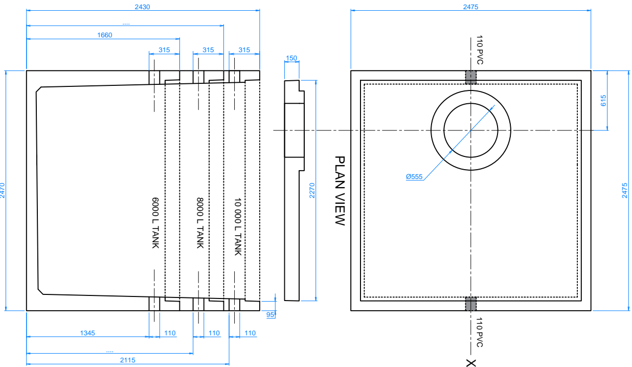
SIDE SECTION X SEPTIC OR WATER TANK
