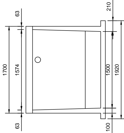
CONSERVANCY TANK SIDE SECTION Y-Y
