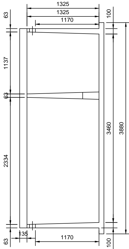
CONSERVANCY TANK SIDE SECTION X-X
